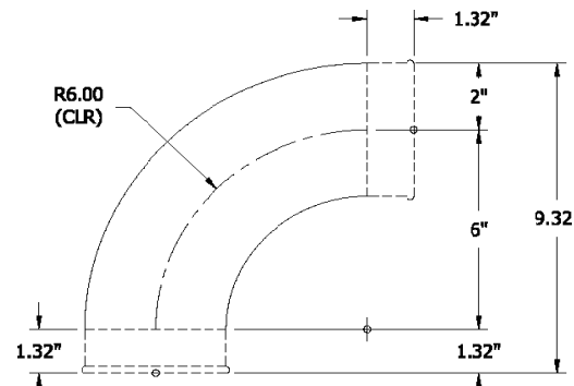
Example shown: 4" 90° Elbow 1.5 CLR=6"
